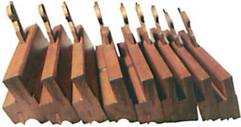
48. A full set of nine graduated side beads by MOSELEY same owner, F (100-140)
