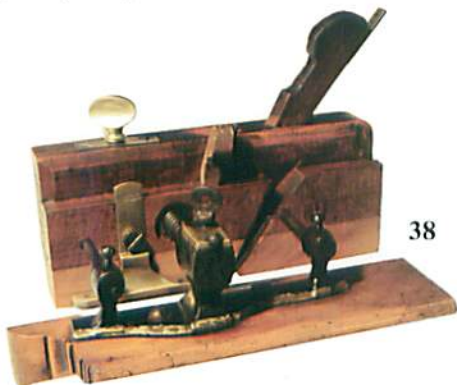
38. A KIMBERLEY sash fillister, G++ (100-150)
