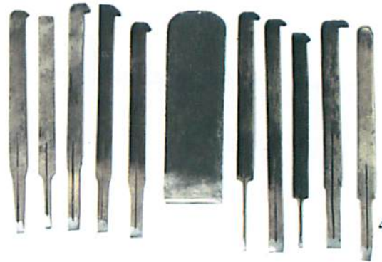
443. A good collection of 18th Century iron blades. A tothing iron by P.LAW , six plough irons by MOTTRAM , two by JAMSCOM and two by P.LAW (30-50)
