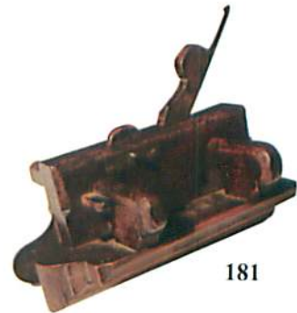
181. An extremely elegant 18th Century sash fillister, single piece skate, unusual looking wooden depth stop and lovely flowing design, G++ (70-100)
