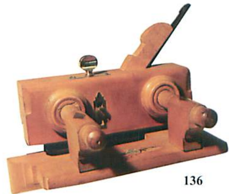
136. A beech WILLIAM MARPLES screwstem plough in mint condition, F (50-80)
